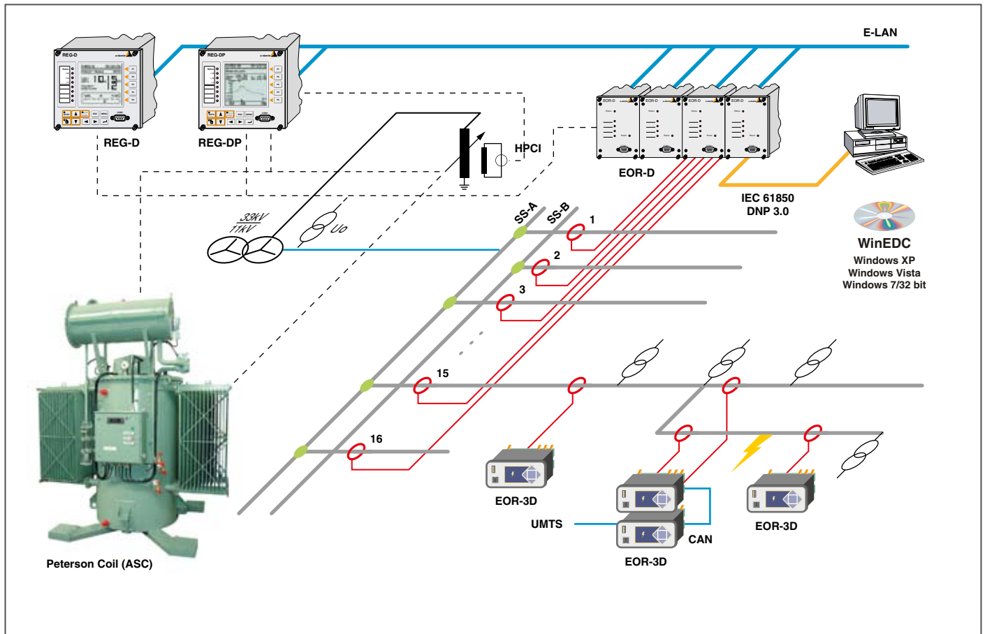
Fig. 2: Combined earth-fault detection and short circuit indicator with high power current injection
