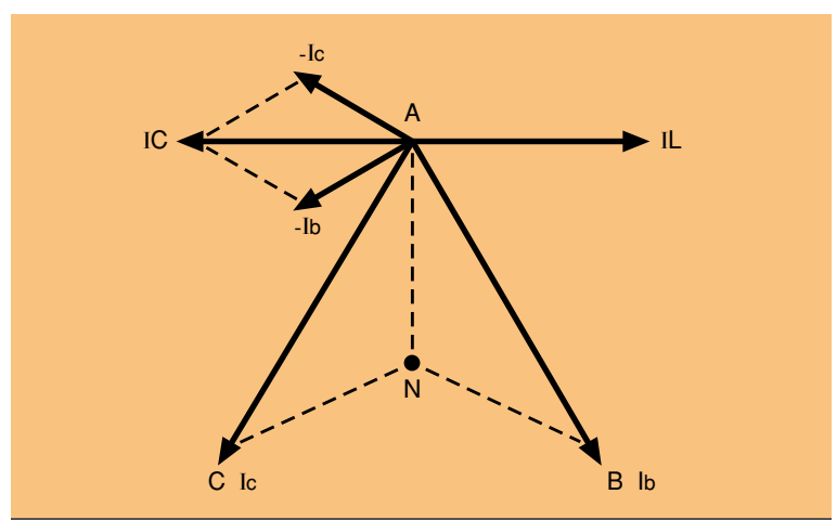
Fig. 1a: Current vectors for A phase fault
