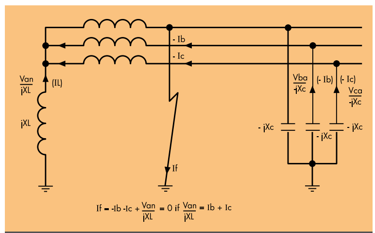
Fig. 1: Current distribution in Petersen Coil earthed system
