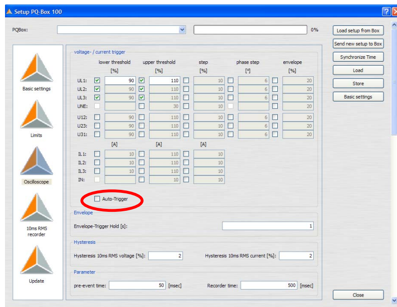
Auto-Trigger check box for Oscilloscope Events.
